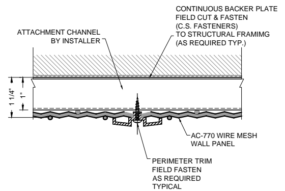
2 PANEL JOINT DETAIL AC-770-FS1
