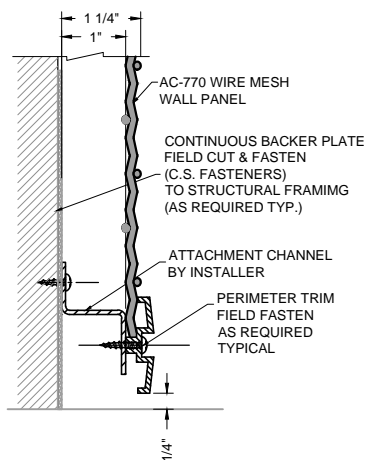
5 PERIMETER DETAIL (BASE) AC-770-FB1
