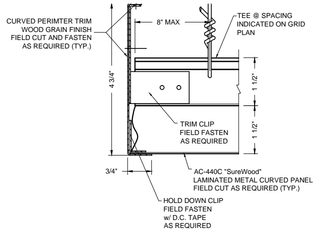
2 PERIMETER DETAIL AC-440C-PFC2
