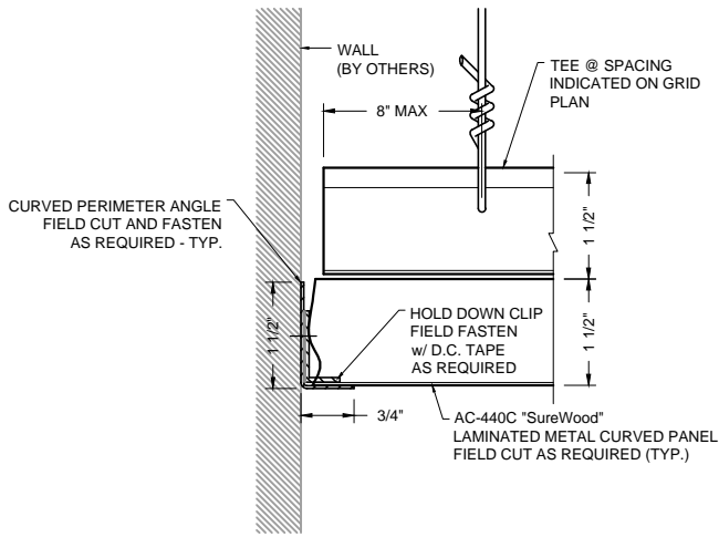
1 PERIMETER DETAIL AC-440C-PFC1
