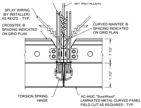
1 PANEL JOINT DETAIL AC-440C-PJ1
