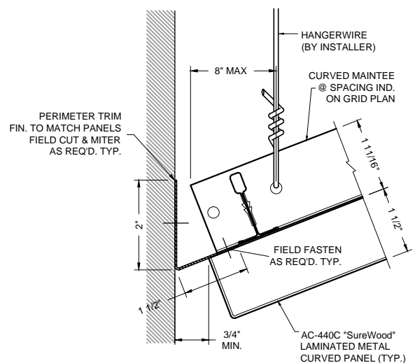
6 PERIMETER DETAIL AC-440C-P6
