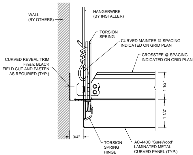
1 PANEL JOINT DETAIL AC-440C-PJ1
