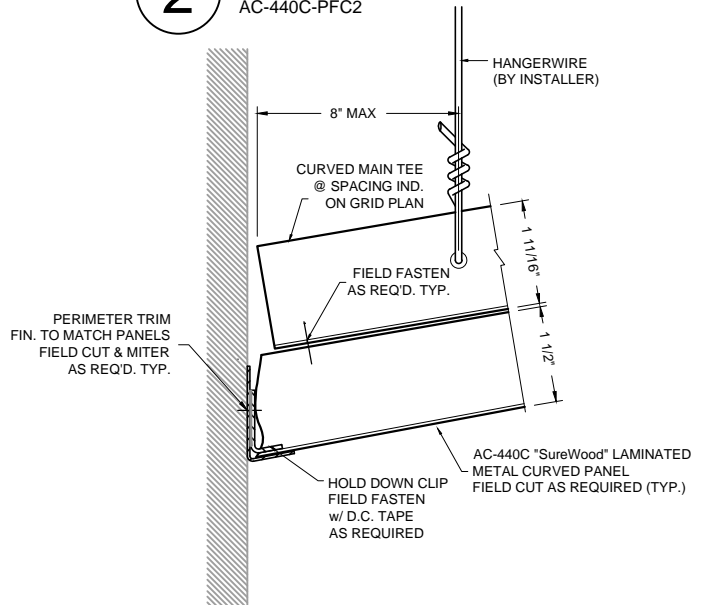
4 PERIMETER DETAIL AC-440C-PFC4
