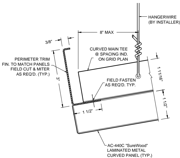
3 PERIMETER DETAIL AC-440C-P2
