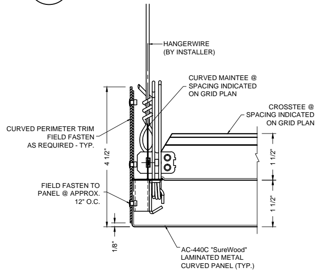
4 PERIMETER DETAIL AC-440C-P4
