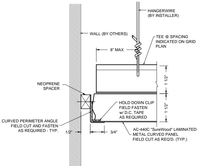
3 PERIMETER DETAIL AC-440C-PFC3
