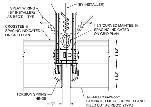
2 PANEL JOINT DETAIL AC-440C-PJ2
