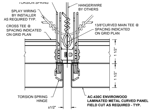
2 PANEL JOINT DETAIL AC-430C-PJ2
