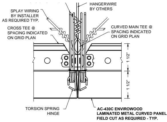
1 PANEL JOINT DETAIL AC-430C-PJ1
