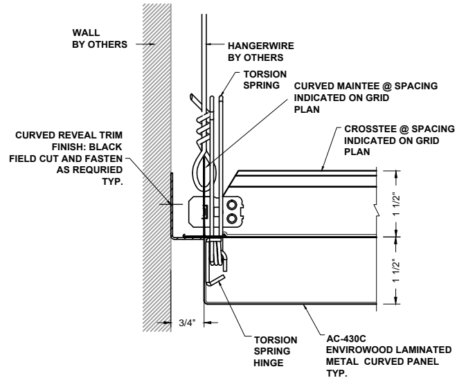
4 PERIMETER DETAIL AC-430C-P2
