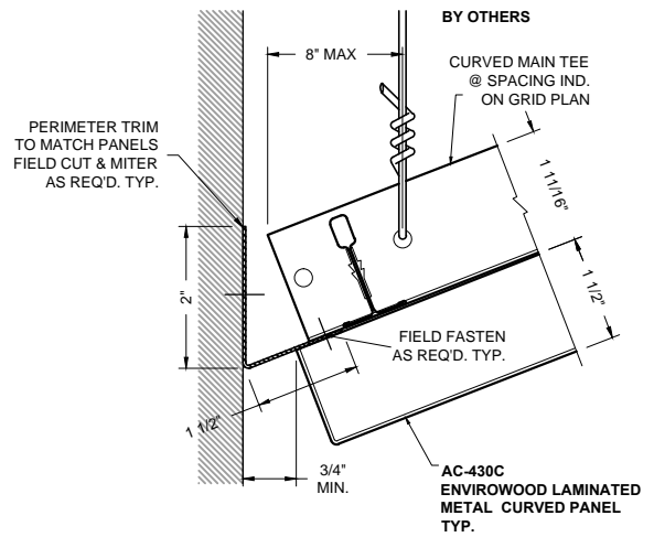
2 PERIMETER DETAIL AC-430C-P6
