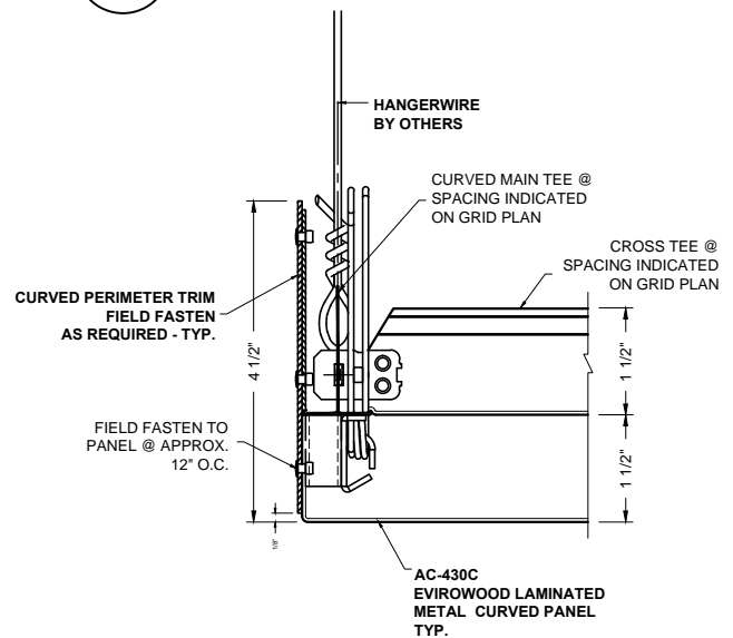
6 PERIMETER DETAIL AC-430C-P4
