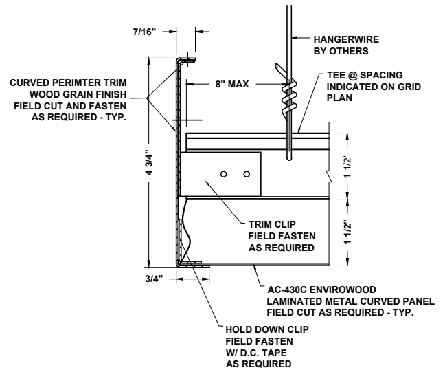
4 PERIMETER DETAIL AC-430C-PFC2
