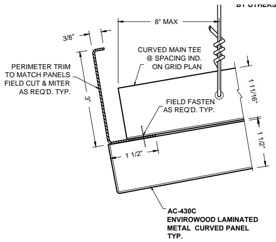
1 PERIMETER DETAIL AC-430C-P5
