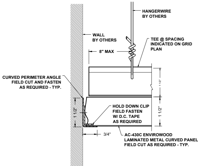
3 PERIMETER DETAIL AC-430C-PFC1
