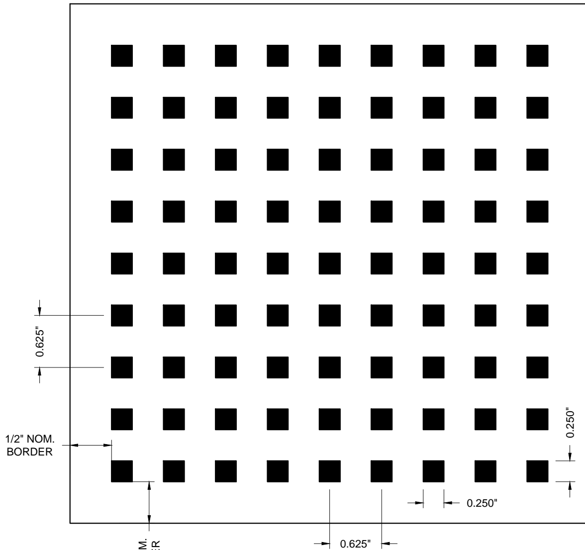
PERFORATION S250-16-1 1/4" SQUARE @ 5/8" STRAIGHT CENTERS (16% OPEN)
