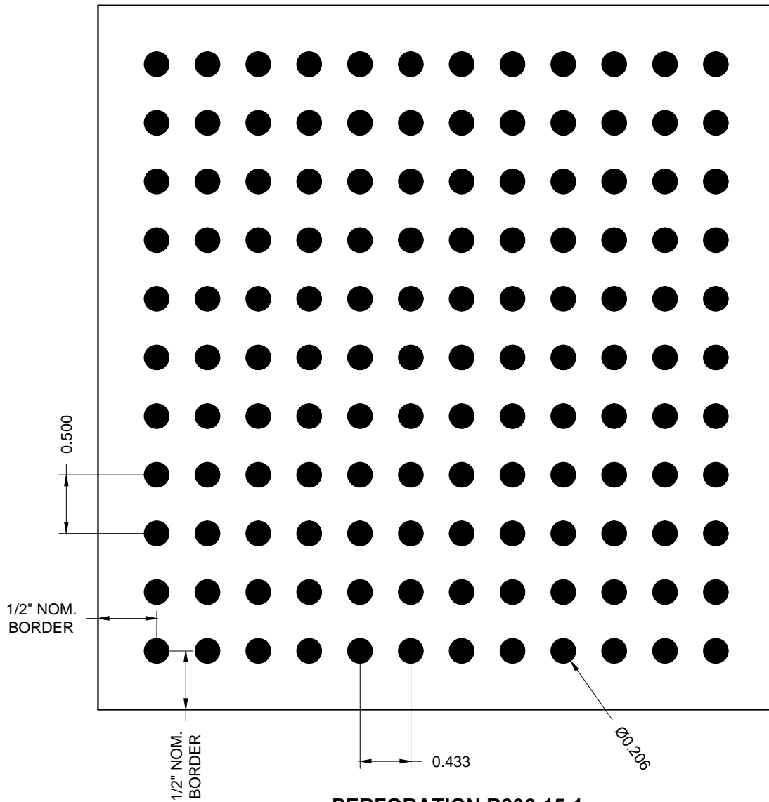
PERFORATION R206-15-1 .206 DIA. HOLES @ .433 x .500" STRAIGHT CENTERS (15% OPEN)
