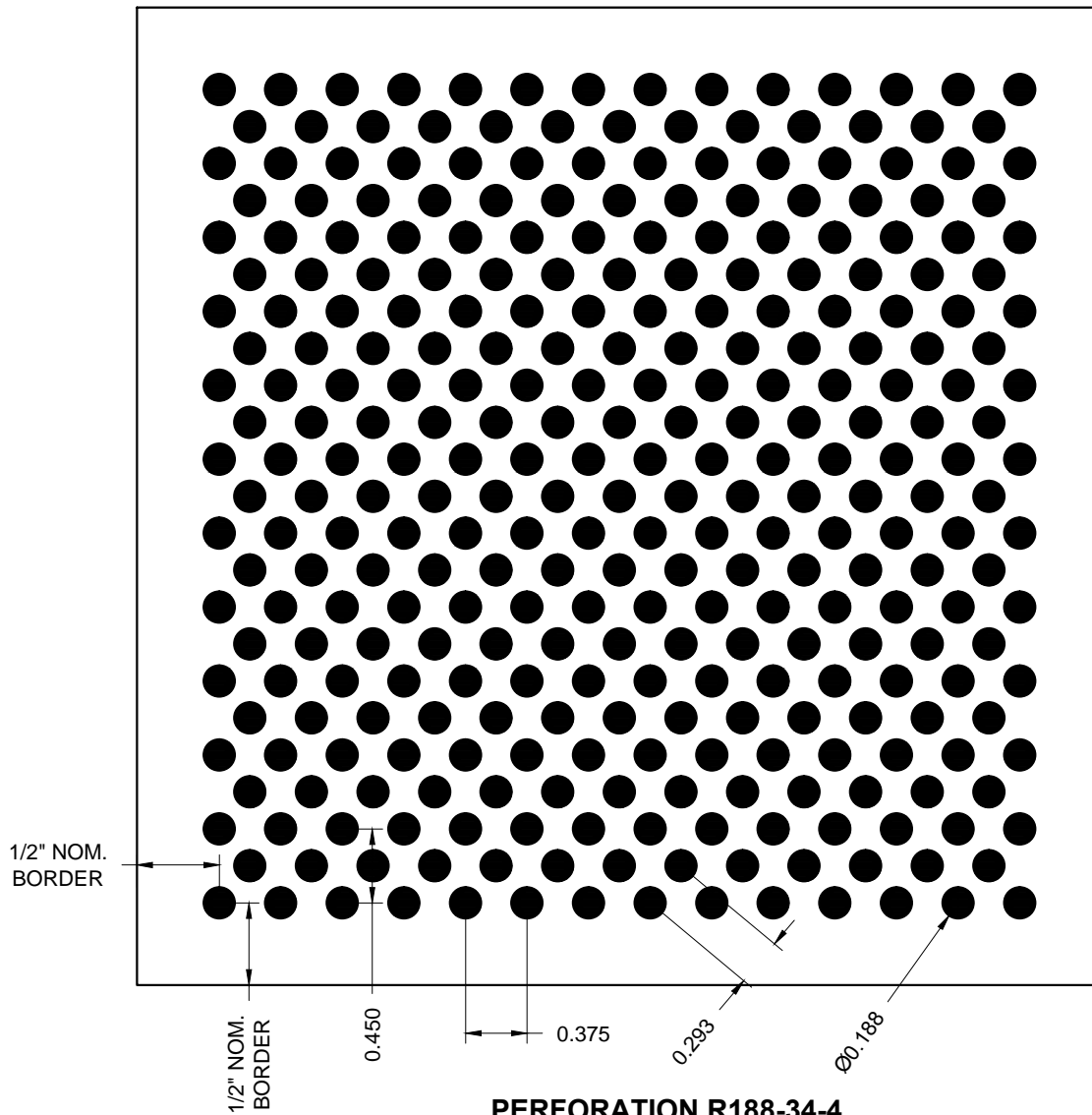
PERFORATION R188-34-4 .188 DIA. HOLES @ .293 CUSTOM STAGGERED CENTERS (34% OPEN)
