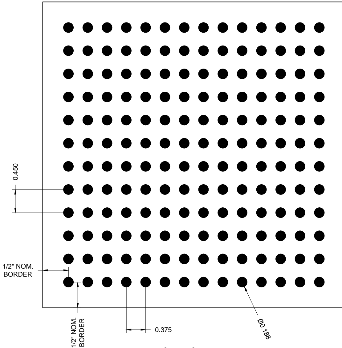
PERFORATION R188-17-1 .188 DIA. HOLES @ .375 x .450" STRAIGHT CENTERS (17% OPEN)
