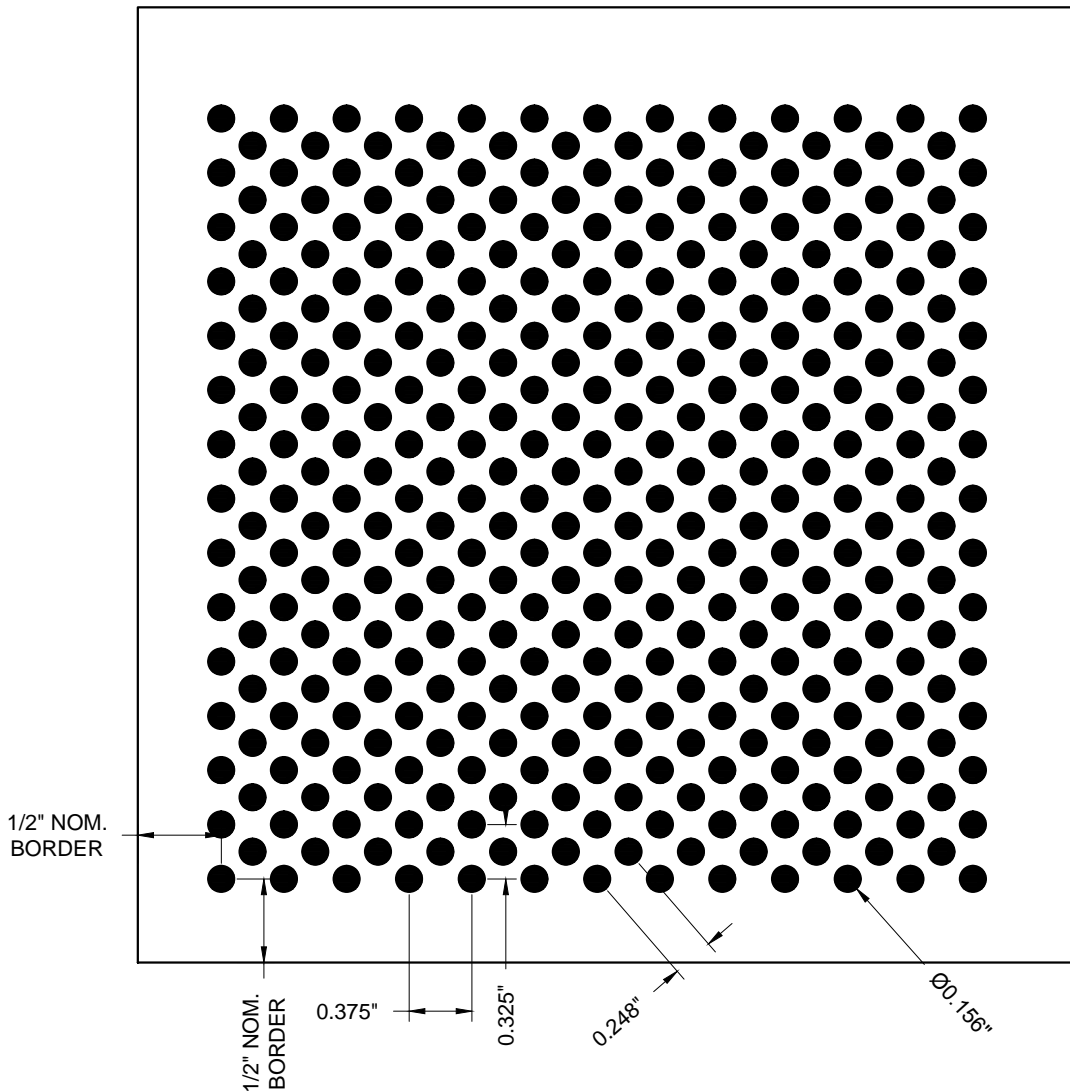
PERFORATION R156-31-4 .156" DIA. HOLES @ .248" CUSTOM STAGGERED CENTERS (16% OPEN)
