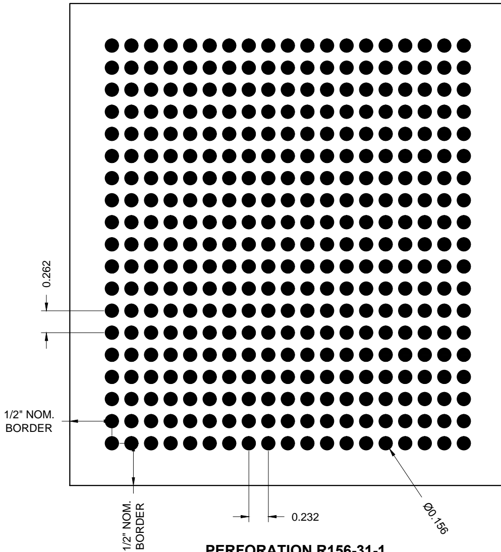
PERFORATION R156-31-1 .156 DIA. HOLES @ .232 x .262 STRAIGHT CENTERS (31% OPEN)
