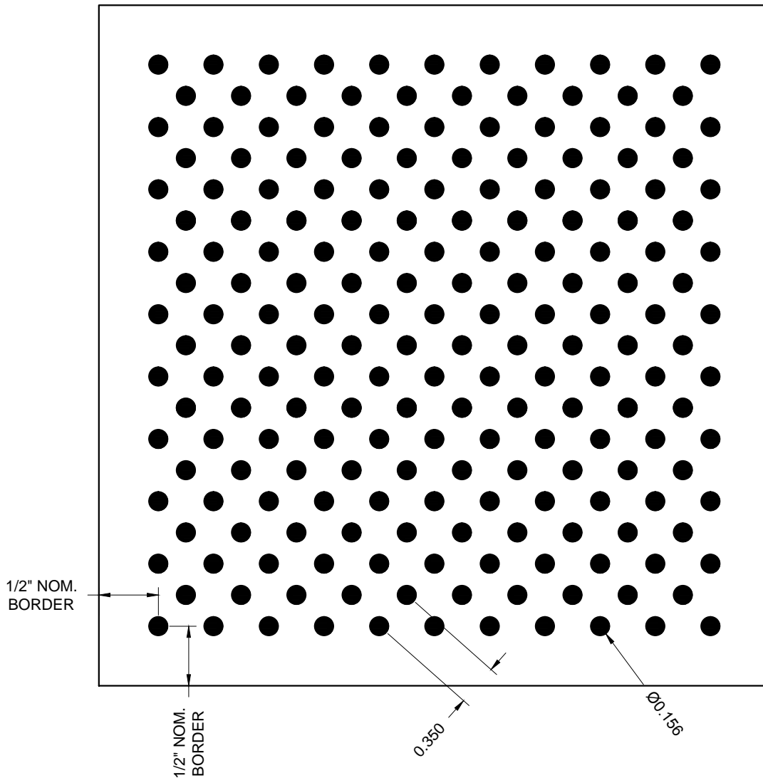
PERFORATION R156-16-4 .156 DIA. HOLES @ .350 CUSTOM STAGGERED CENTERS (16% OPEN)
