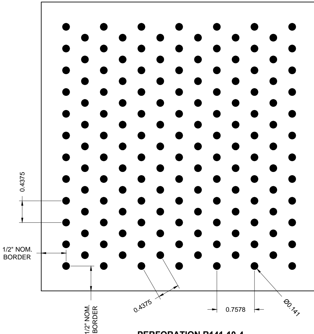
PERFORATION R141-10-4 .141" DIA. HOLES @ .4375" STAGGERED CENTERS (10% OPEN)
