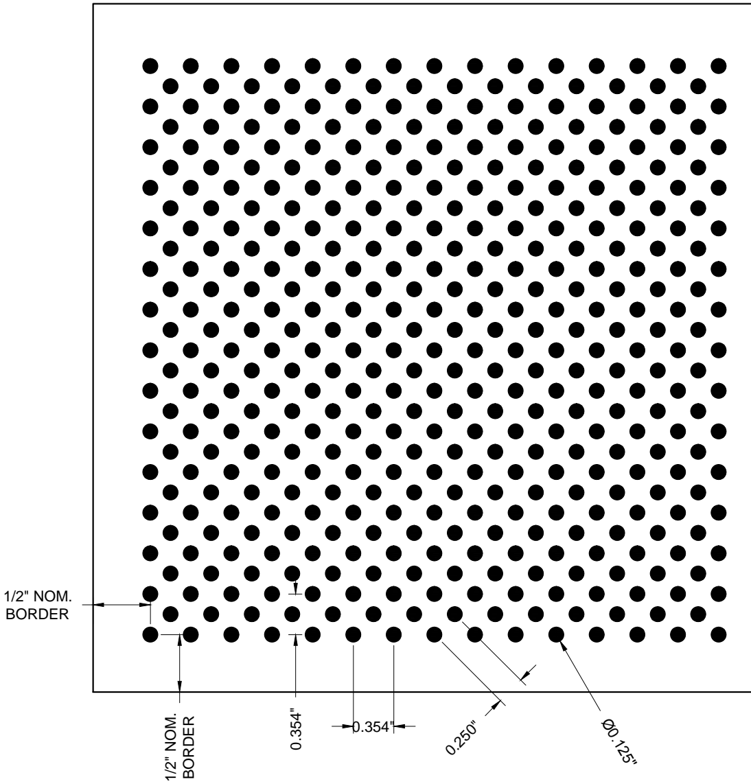
PERFORATION R125-20-3 .125 DIA. HOLES @ .250" CUSTOM STAGGERED CENTERS (20% OPEN)
