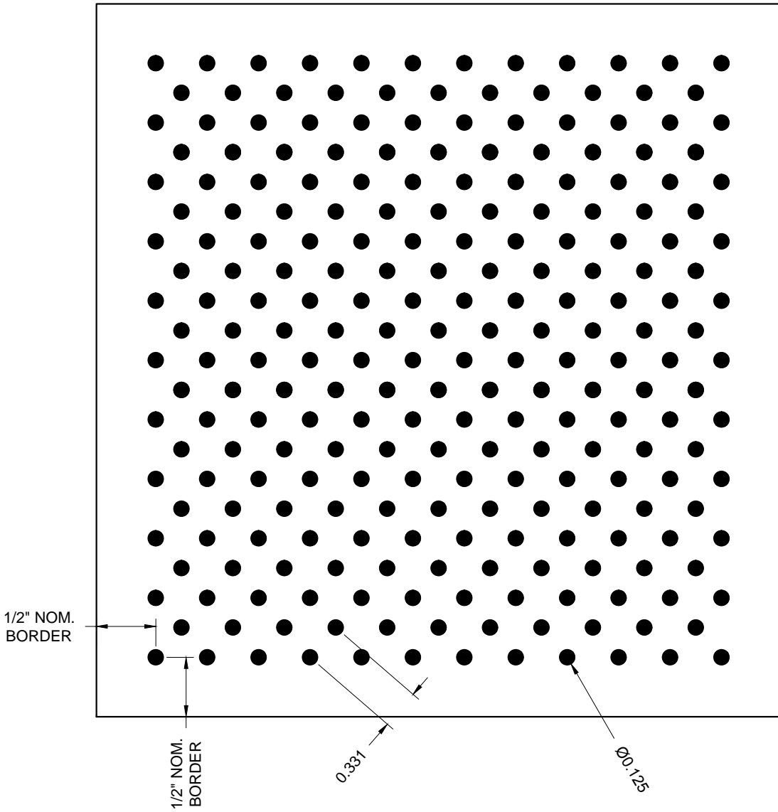
PERFORATION R125-12-4 .125 DIA. HOLES @ .331 CUSTOM STAGGERED CENTERS (12% OPEN)
