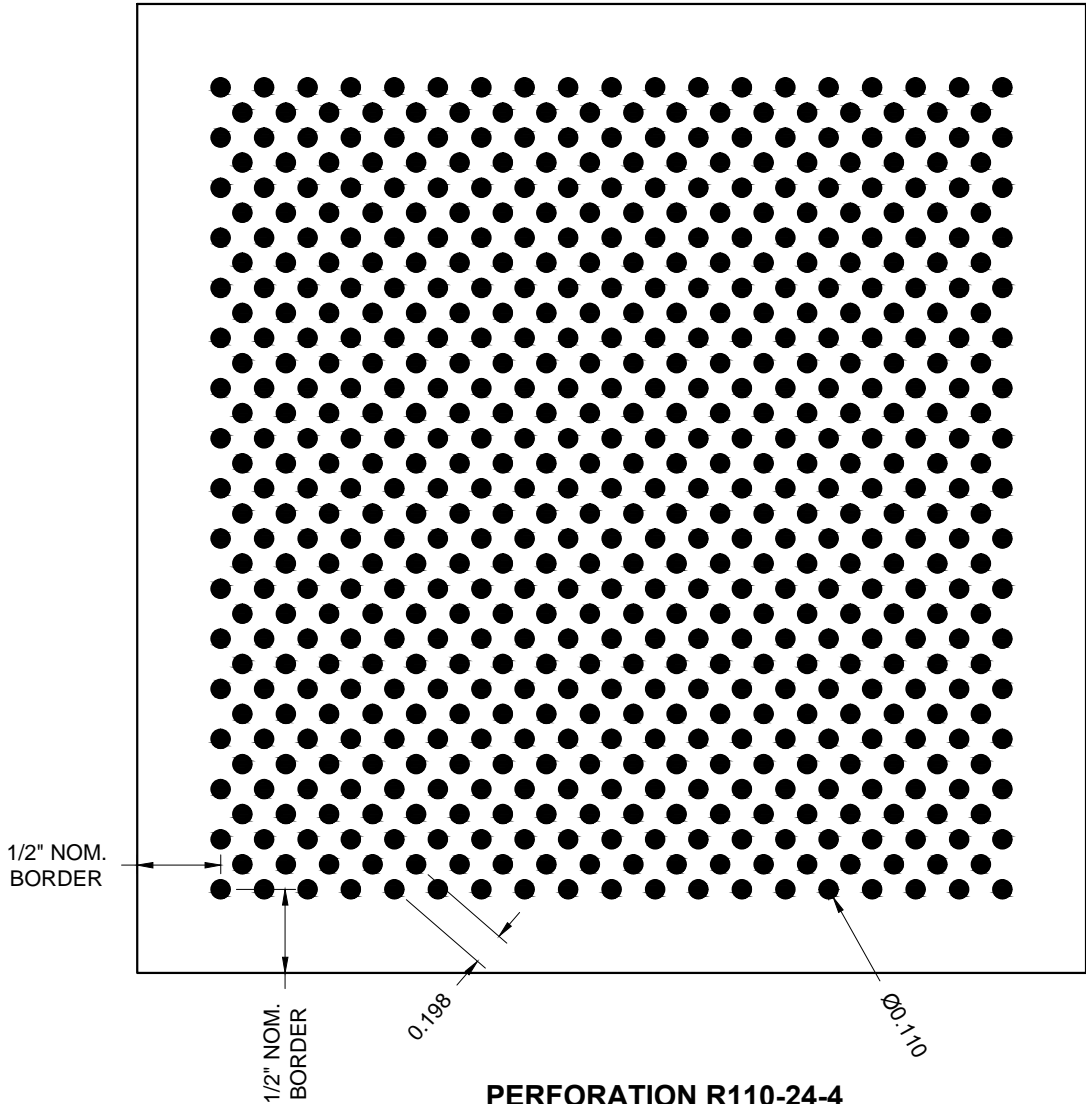
PERFORATION R110-24-4 .110 DIA. HOLES @ .198 CUSTOM STAGGERED CENTERS (24% OPEN)
