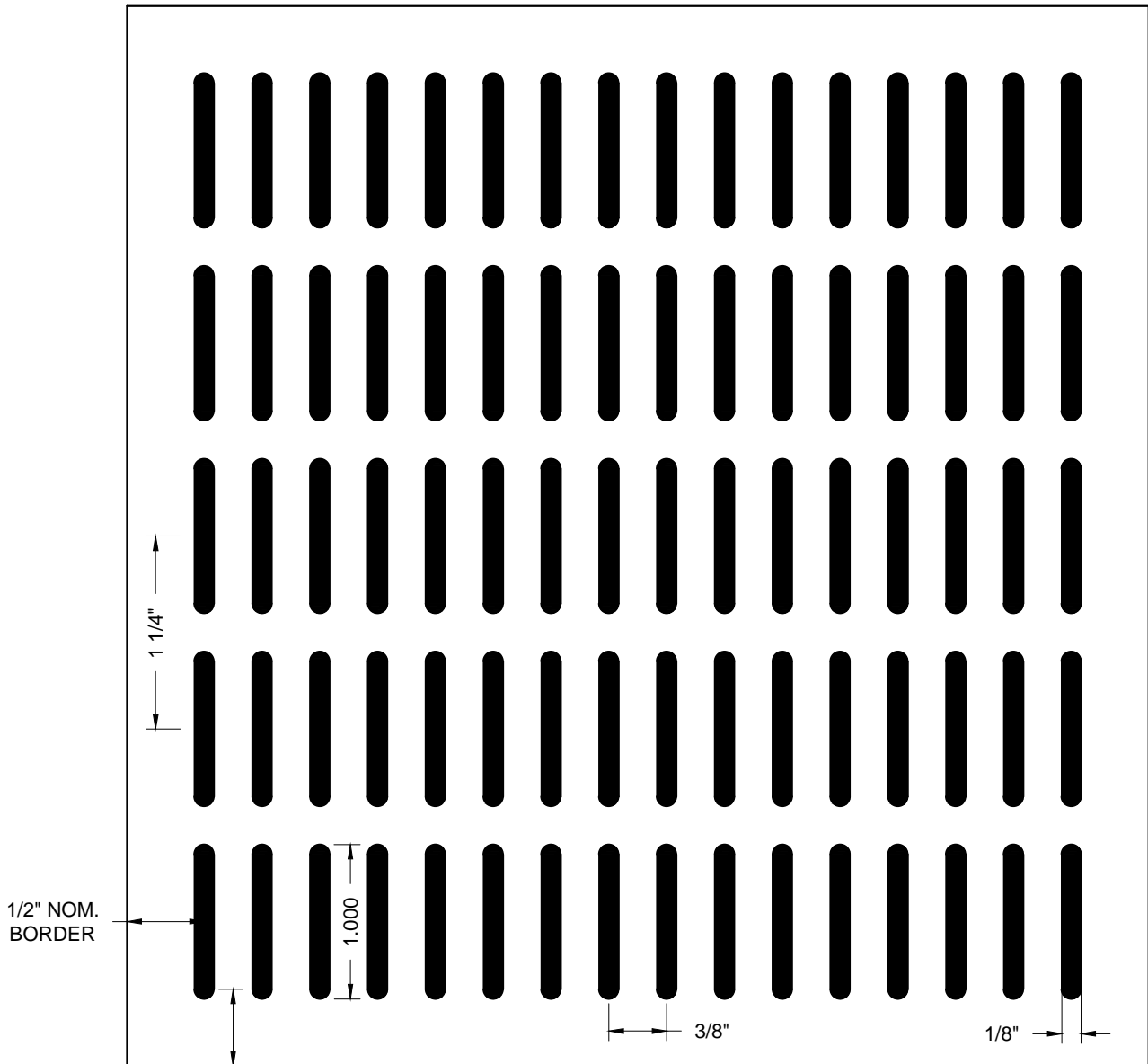
PERFORATION, OB125x100-26-1 1/8" x 1.00 OBROUND SLOT @ 3/8" x 1-1/4" STRAIGHT CENTERS (26% OPEN)
