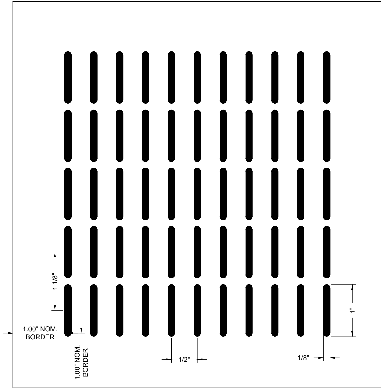
PERFORATION OB-125x100-22-1 1/8" x 1.000" OBROUND SLOT @ 1/2" x 1-1/8" STRAIGHT CENTERS (22% OPEN)
