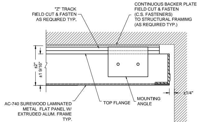
2 PANEL JOINT DETAIL AC-740-FS1
