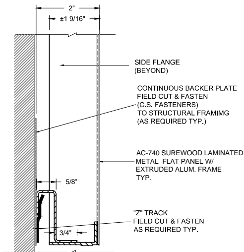
5 PERIMETER DETAIL (BASE) AC-740-FB1
