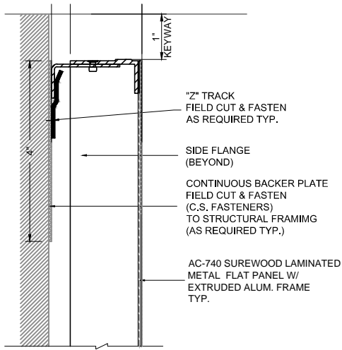
1 PERIMETER DETAIL (TOP) AC-740-FT1
