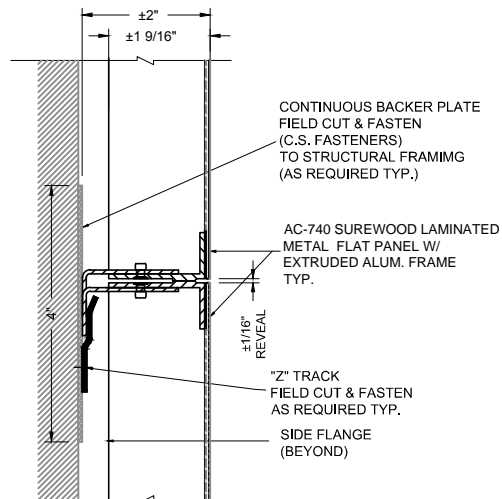
3 PANEL JOINT DETAIL AC-740-FM1
