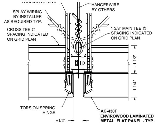
2 PANEL JOINT DETAIL AC-430F-PJ2
