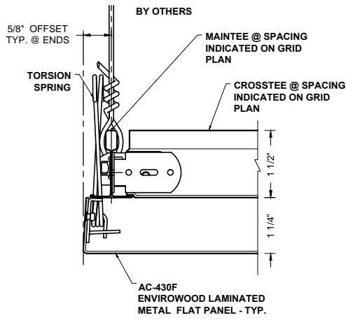
1 PERIMETER DETAIL AC-430F-P5
