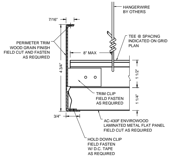
4 PERIMETER DETAIL AC-430F-PFC2
