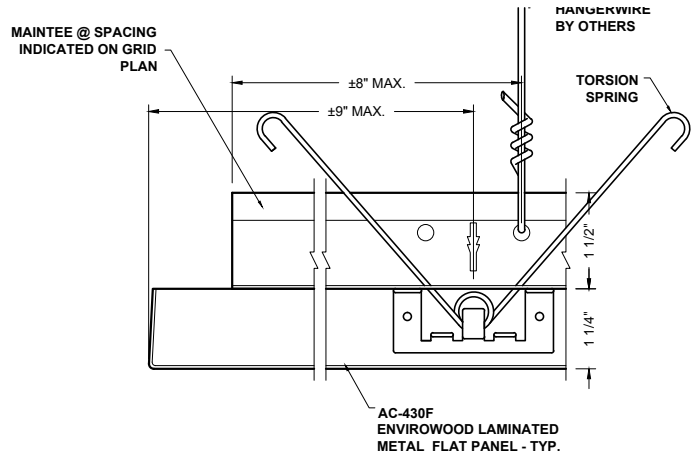
2 PERIMETER DETAIL AC-430F-P6
