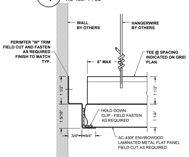
4 PERIMETER DETAIL AC-430F-PFC2
