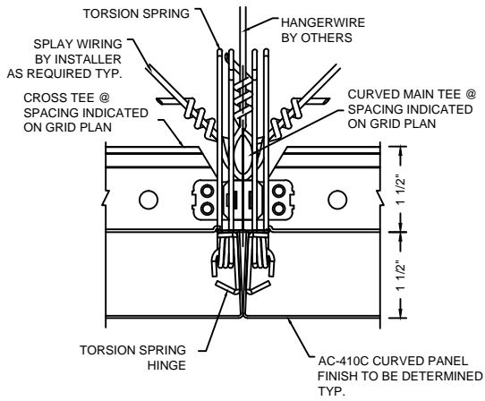
1 PANEL JOINT DETAIL AC-410C-PJ1
