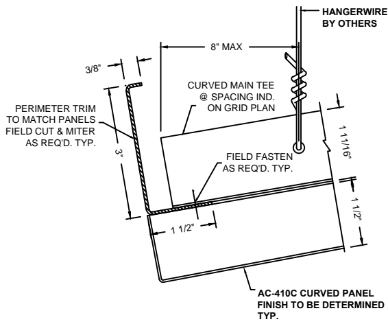
1 PERIMETER DETAIL AC-410C-P5
