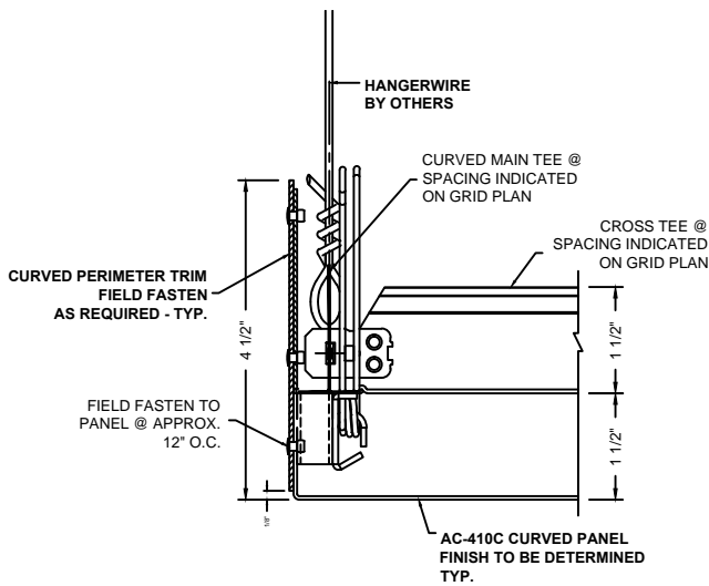
3 PERIMETER DETAIL AC-410C-P4
