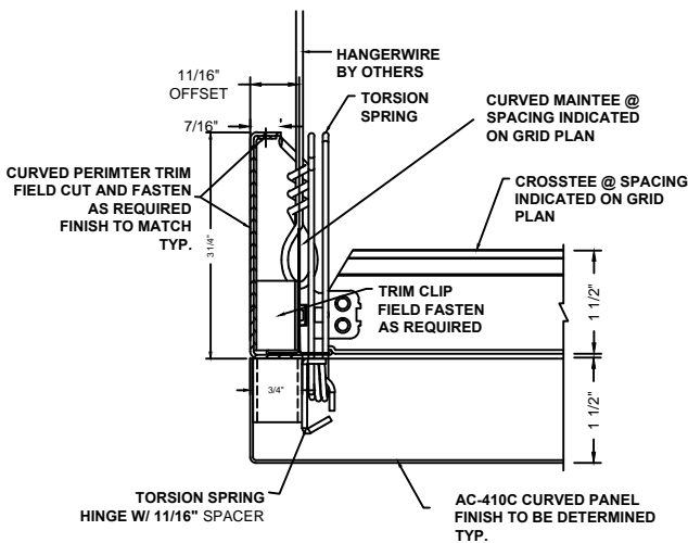
3 PERIMETER DETAIL AC-410C-P4
