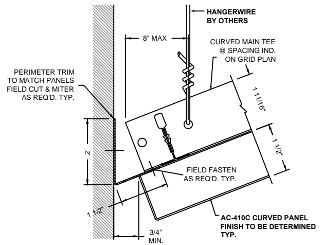
2 PERIMETER DETAIL AC-410C-P6
