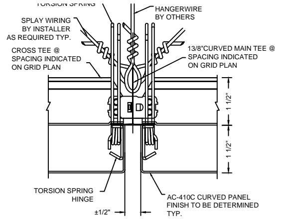
2 PANEL JOINT DETAIL AC-410C-PJ2
