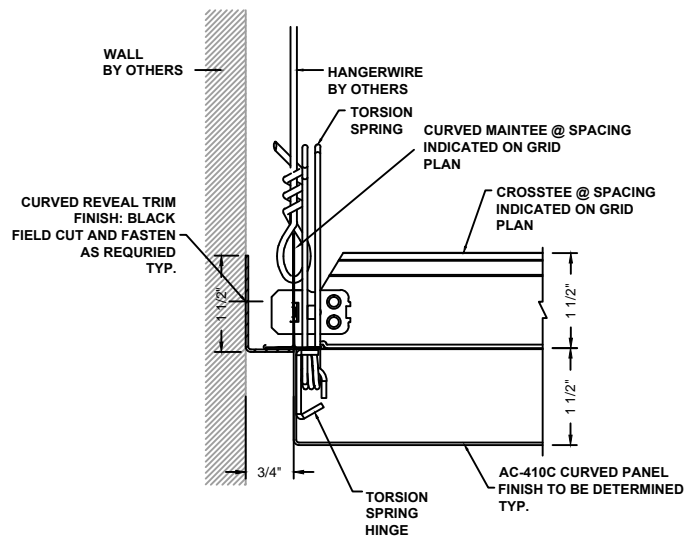
4 PERIMETER DETAIL AC-410C-P2
