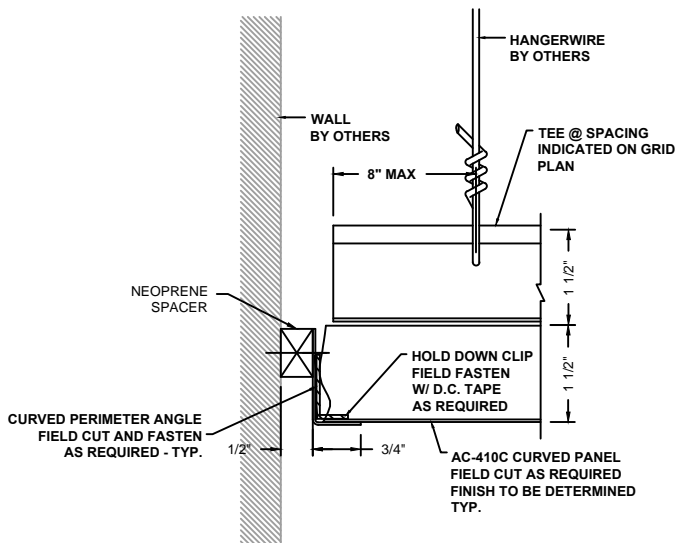
5 PERIMETER DETAIL AC-410C-PFC3
