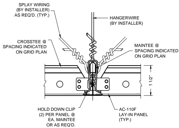
1 PANEL JOINT DETAIL AC-110F-PJ1
