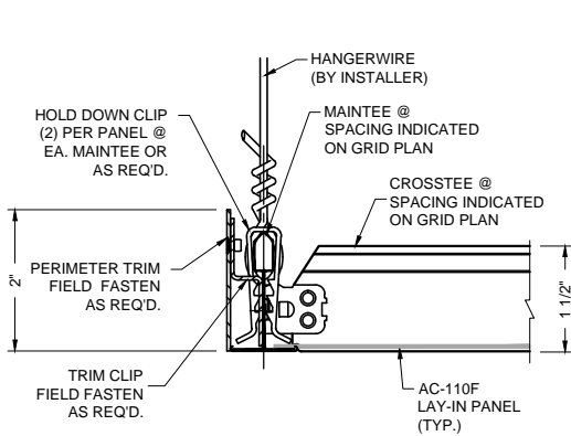
3 PERIMETER DETAIL AC-110F-P2
