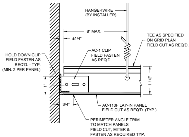
5 PERIMETER DETAIL AC-110F-PFC1
