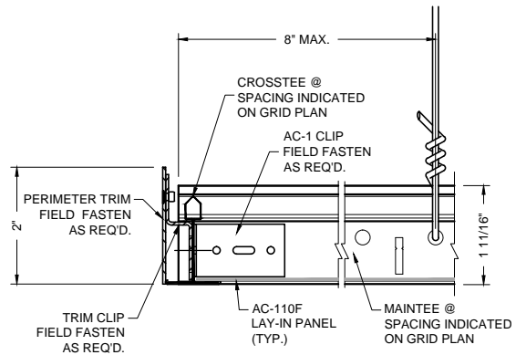
4 PERIMETER DETAIL AC-110F-P3
