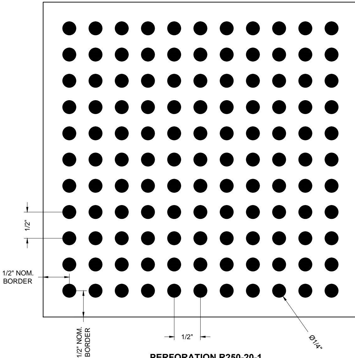
PERFORATION R250-20-1 1/4" DIA. HOLES @ 1/2" STRAIGHT CENTERS (20% OPEN)
