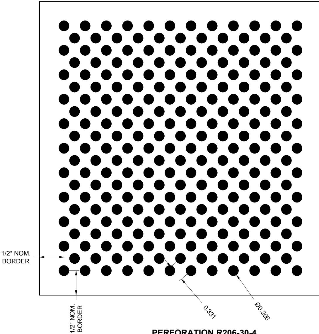
PERFORATION R206-30-4 .206 DIA. HOLES @ .331 CUSTOM STAGGERED CENTERS (30% OPEN)
