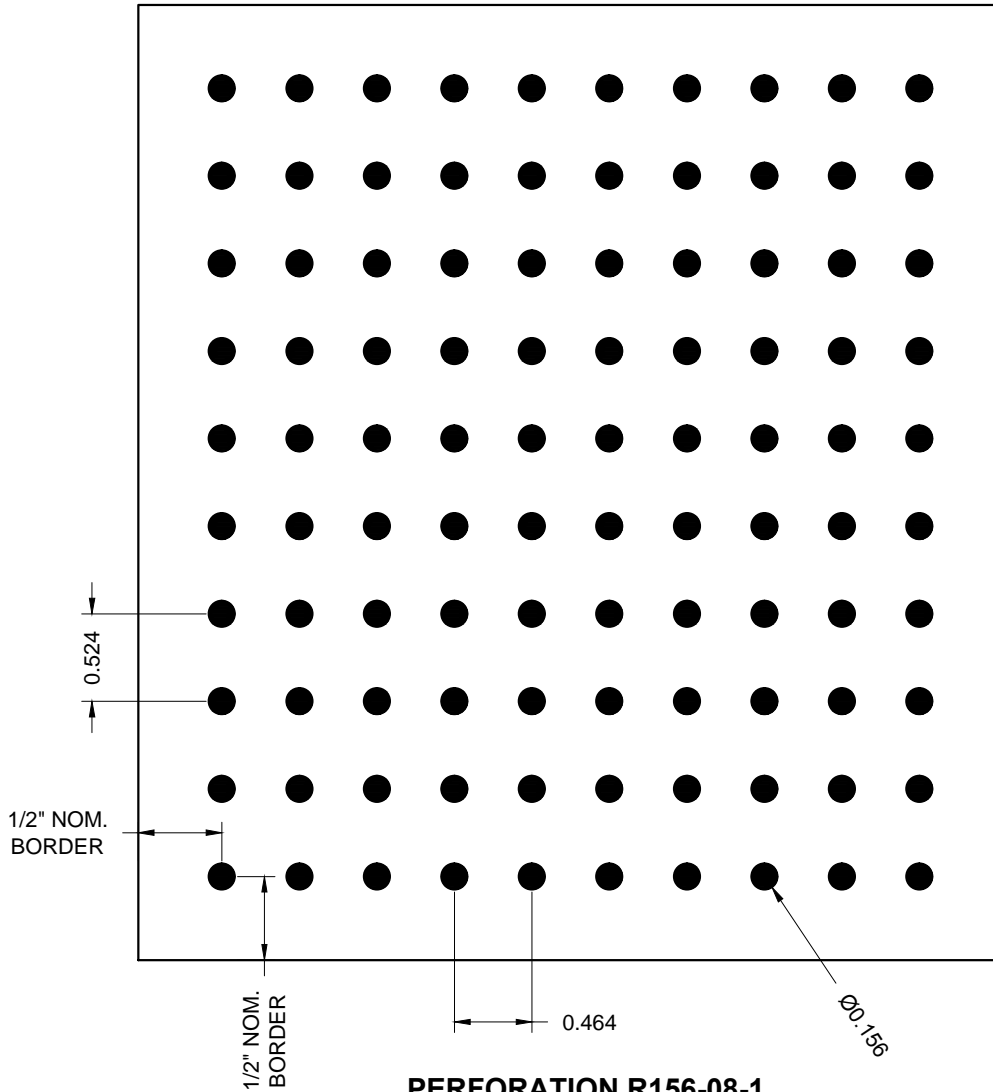
PERFORATION R156-08-1 .156 DIA. HOLES @ .464 x .524 STRAIGHT CENTERS (8% OPEN)
