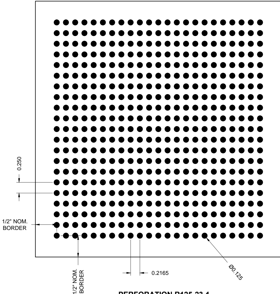
PERFORATION R125-23-1 .125 DIA. HOLES @ .2165 x .250 STRAIGHT CENTERS (23% OPEN)
