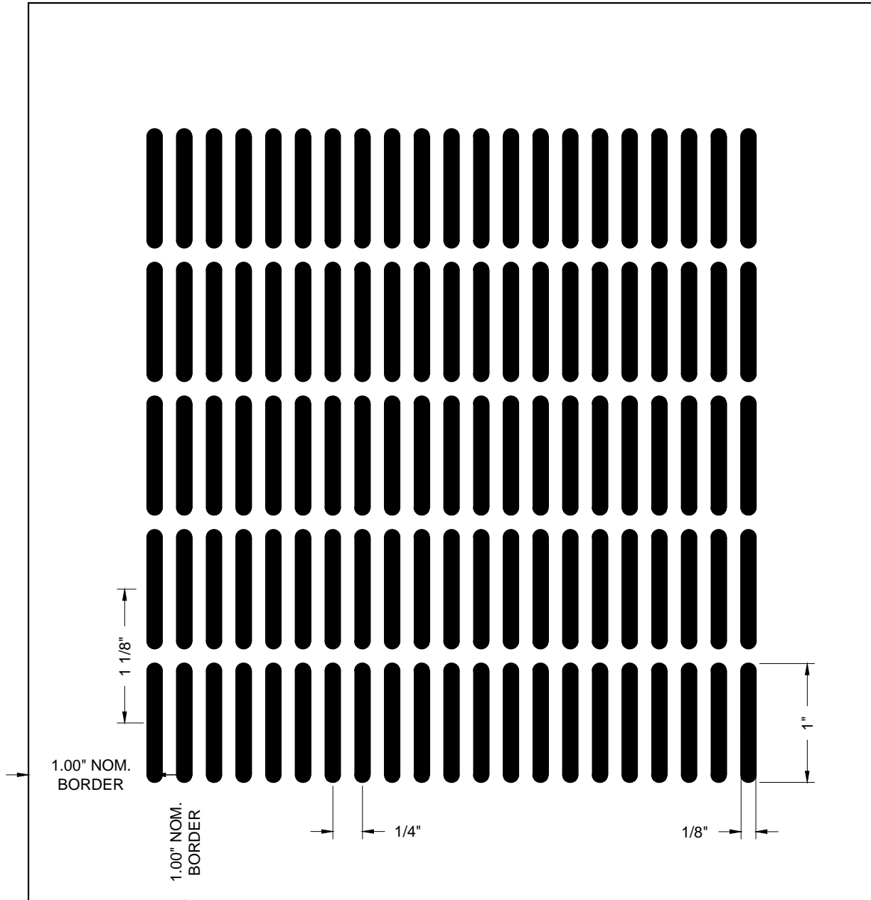
PERFORATION OB,125x1000-43-1 1/8" x 1.00 OBROUND SLOT @ 1/4" x 1-1/8" STRAIGHT CENTERS (43% OPEN)
