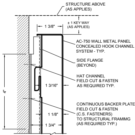
1 PERIMETER DETAIL (TOP) AC-750-FT1
