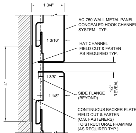
5 PANEL JOINT DETAIL AC-750-FM2
