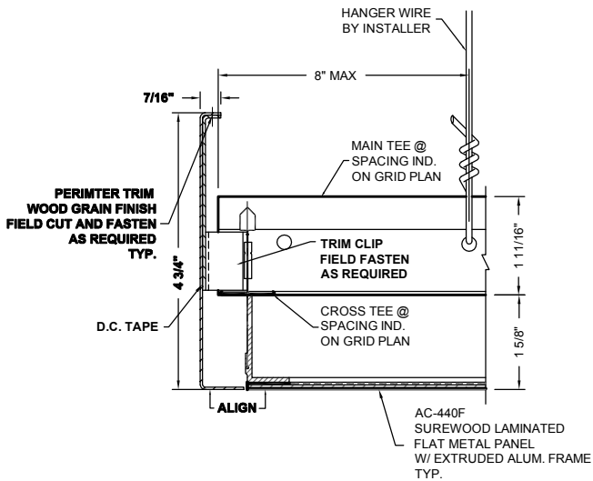
1 PERIMETER DETAIL AC-440F-P6
