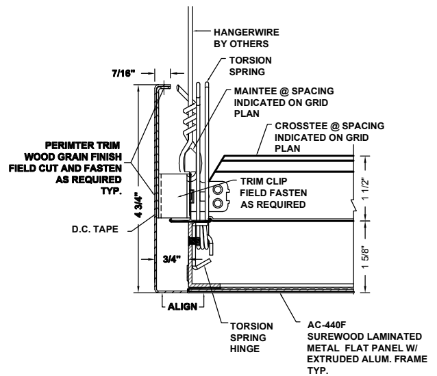
2 PERIMETER DETAIL AC-440F-P1
