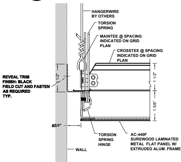
3 PERIMETER DETAIL AC-440F-P2
