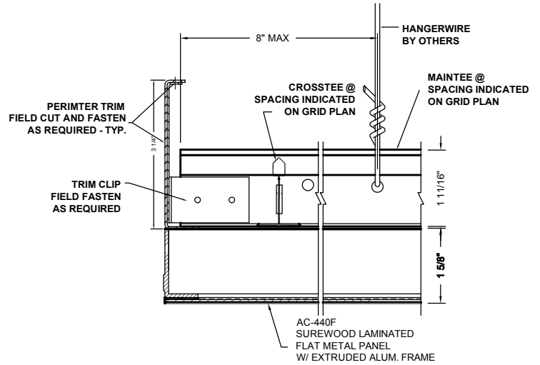
2 PERIMETER DETAIL AC-440F-P7
