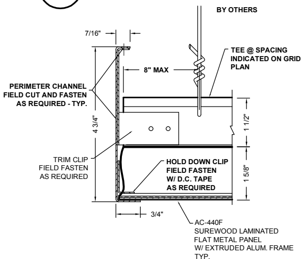
5 PERIMETER DETAIL AC-440F-PFC3
