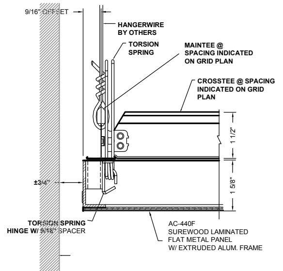
4 PERIMETER DETAIL AC-440F-P3
