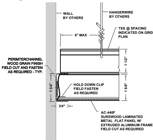
3 PERIMETER DETAIL AC-440F-PFC1
