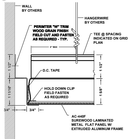
4 PERIMETER DETAIL AC-440F-PFC2
