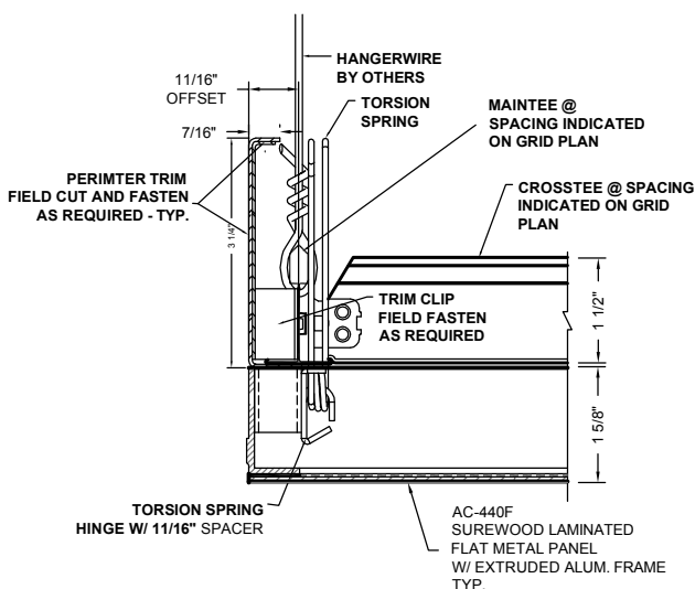
5 PERIMETER DETAIL AC-440F-P4
