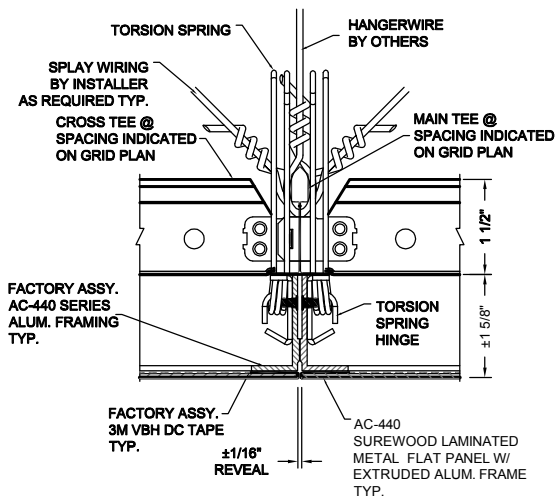
1 PANEL JOINT DETAIL AC-440F-PJ1
