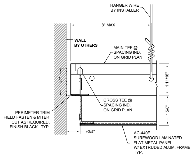
6 PERIMETER DETAIL AC-440F-P5
