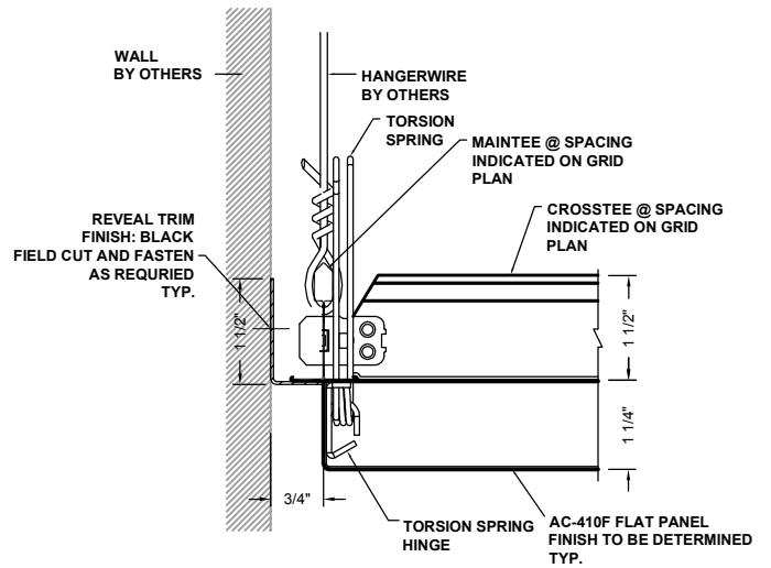
4 PERIMETER DETAIL AC-410F-P2
