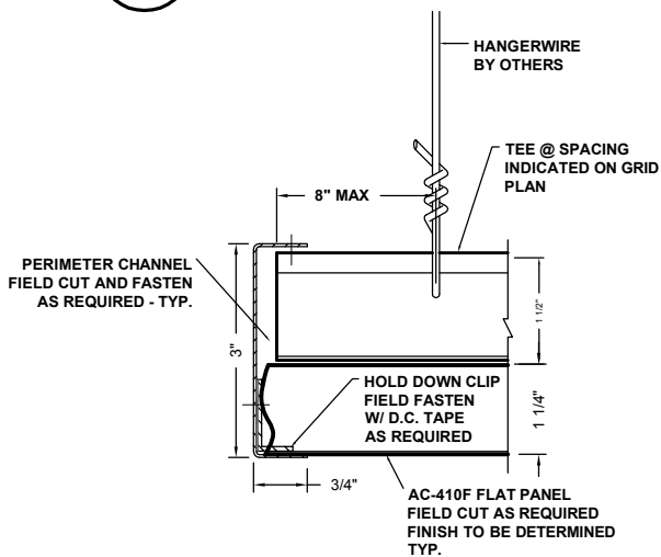
3 PERIMETER DETAIL AC-410F-PFC1
