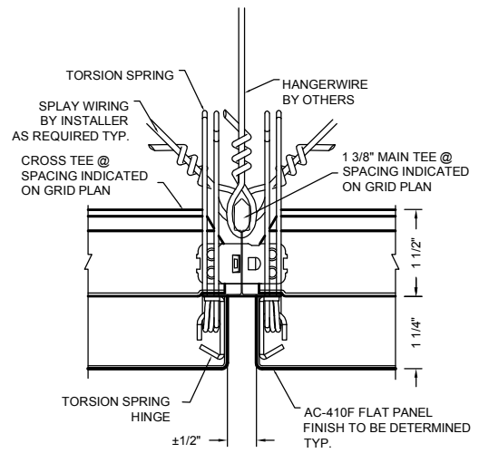
2 PANEL JOINT DETAIL AC-410F-PJ2
