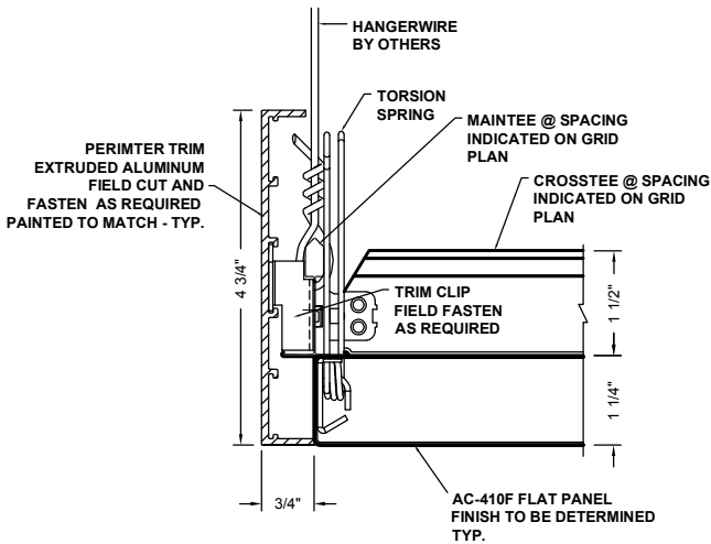
3 PERIMETER DETAIL AC-410F-P1
