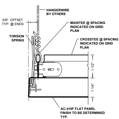
1 PERIMETER DETAIL AC-410F-P5
