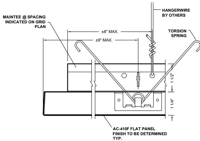
2 PERIMETER DETAIL AC-410F-P6
