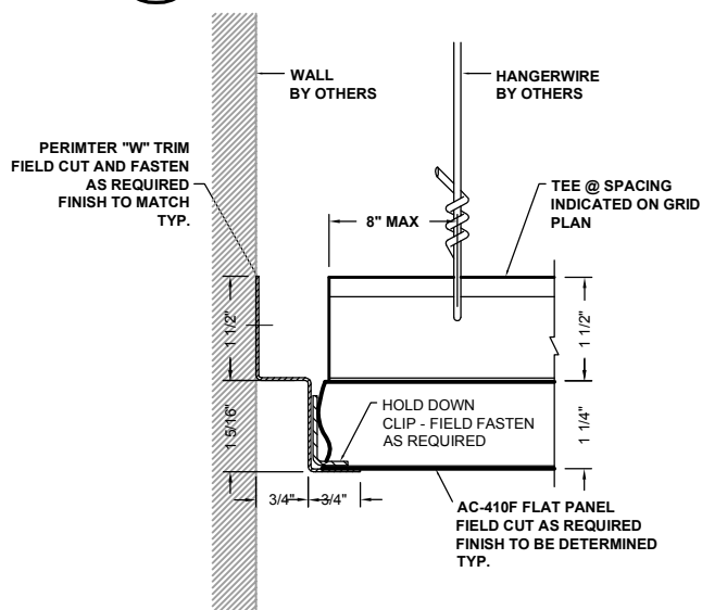
4 PERIMETER DETAIL AC-410F-PFC2
